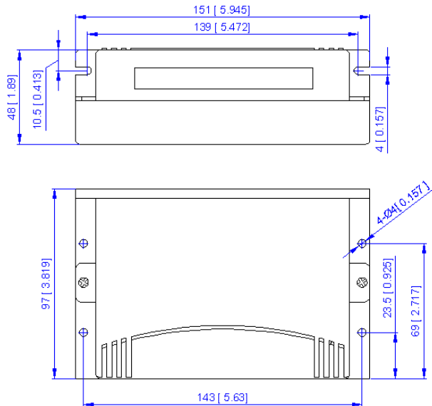
Figure 1: Mechanical specifications
