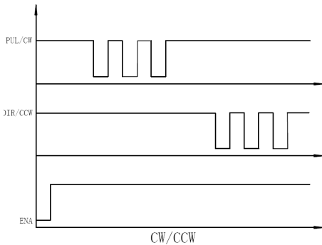
Figure 11: Sequence chart of control signals
