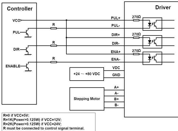
Figure 10: Typical connection
