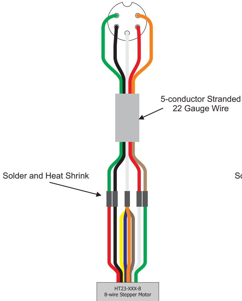
5-pin Connector Set
