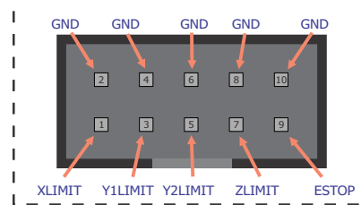
Figure 3: LIMITS Header Pin Diagram
