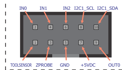
Figure 4: AUX Header Pin Diagram
