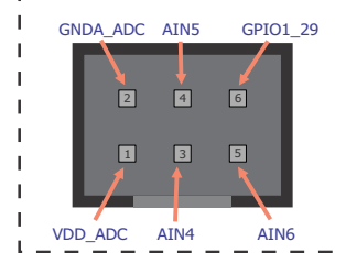
Figure 5: AIN Header Pin Diagram
