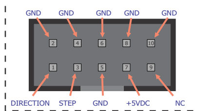
Figure 1: X/Y/Z/A Axis Header Pin Diagram
