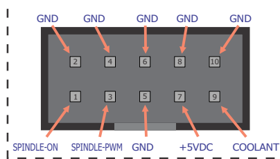
Figure 2: RBX-1 Header Pin Diagram
