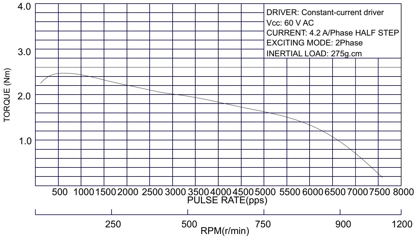
HT23-420-8 Torque Curve
