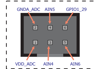
Figure 4: AIN Header Pin Diagram
